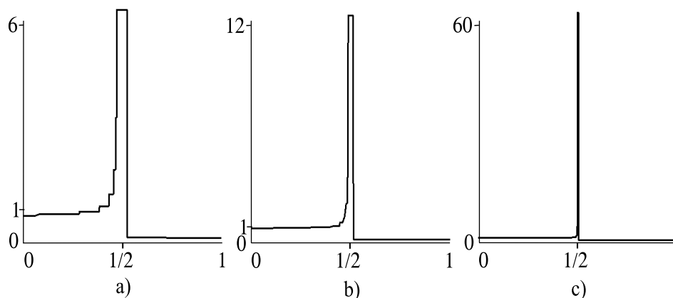
FIGURE 2. W_a -invariant pdf's for a) a = 0.1 , b) a = 0.05 and c) a = 0.01 .
