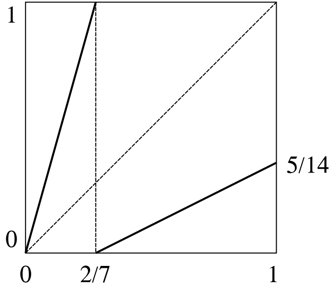
FIGURE 1. Graph of y = f(x) for p = 7/2 and s = 1/2 .
