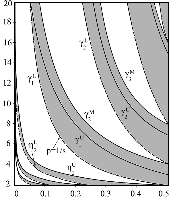
FIGURE 2. The shaded regions are the regions where f has been proven to be eventually expanding for p > 2 and s < 1/2 . If 1 < p \leq 2 or s \geq 1/2 , f is eventually expanding by Proposition 1 and Corollary 1. It is conjectured that f is eventually expanding whenever 1 < p and 0 < s < 1 .
